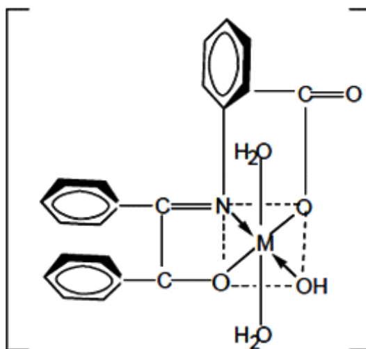
Figure 1: The proposed general Structure of iron (II) and nickel (II) Schiff base complexes
